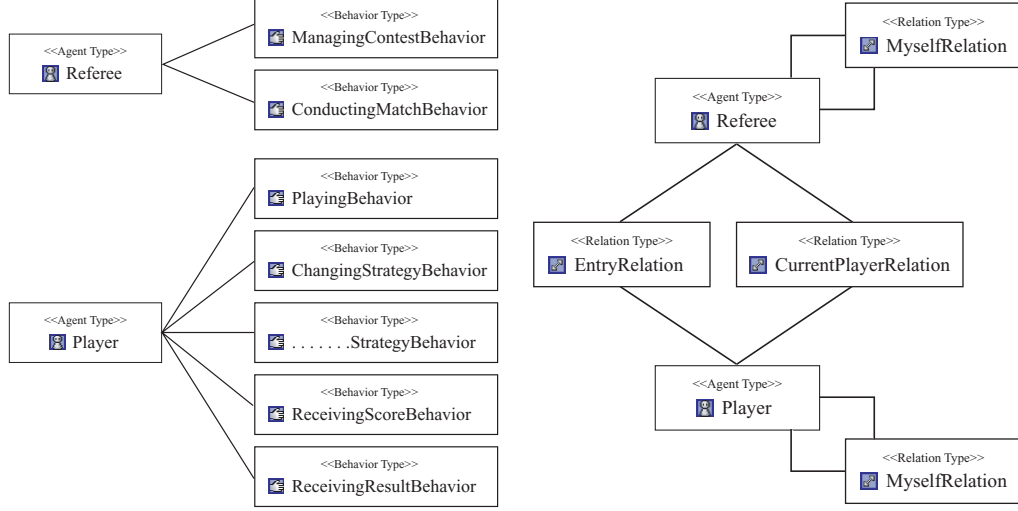
Fig. 9. Class diagram of the extended IPD model
