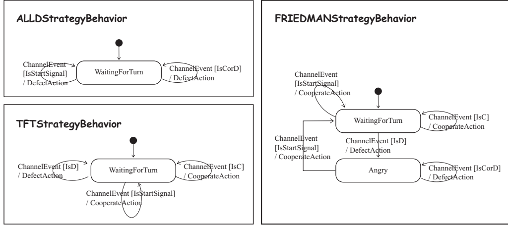
Fig. 10. Statechart diagrams of Strategy Behavior
