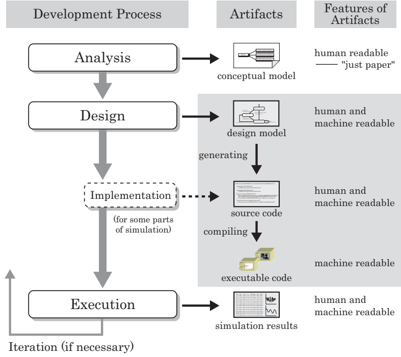
Fig. 15. New Process of Software Development
