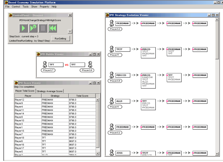
Fig. 12. Screenshot of the extended IPD simulation on BESP
