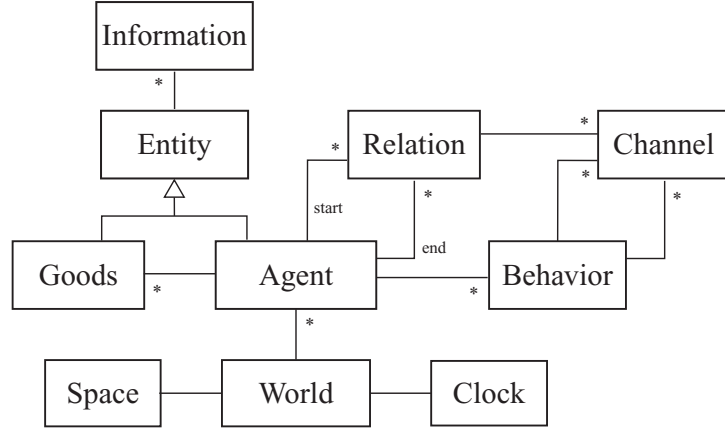
Fig. 3. Major classes of Boxed Economy Foundation Model (BEFM)
