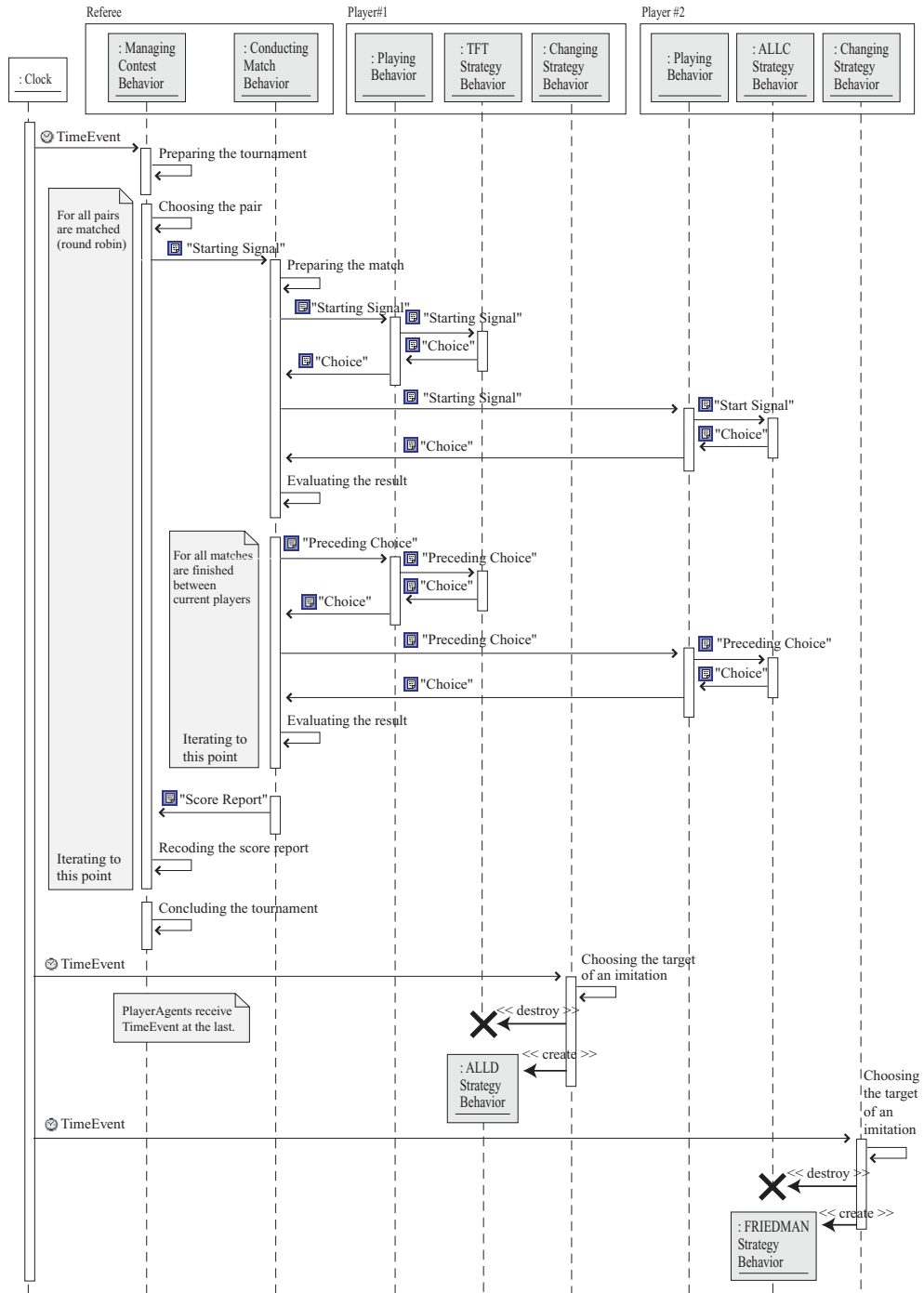
Fig. 11. Communication-sequence diagram of the extended IPD model
