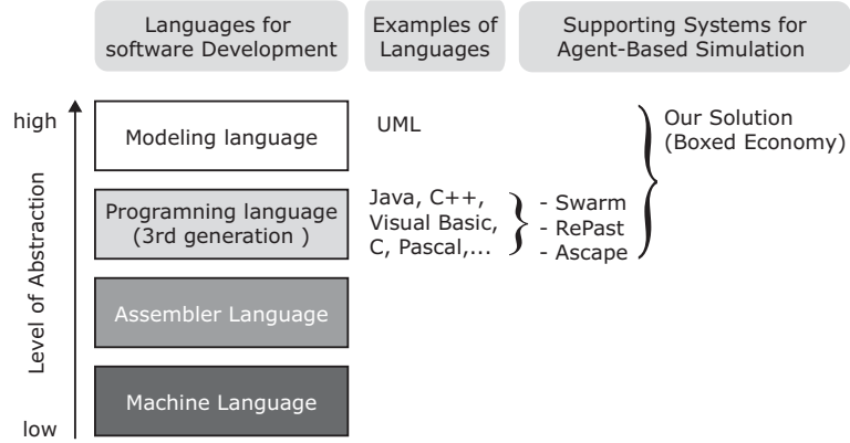
Fig. 13. Level of Abstraction, Languages, and Supporting Systems
