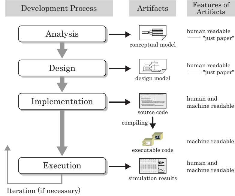
Fig. 14. Traditional Process of Software Development
